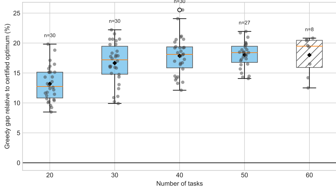
Distribution of Greedy optimality gaps
